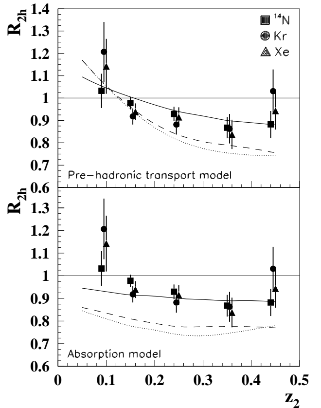
FIG. 1: The ratio R_{2h} as a function of z_2 for ^{14}\text{N} (squares), Kr (circles) and Xe (triangles) with z_1 > 0.5 . Only Selection I was considered. The systematical uncertainty is 2% for all the targets and is independent of z_2 . In the upper panel the curves (solid for ^{14}\text{N} , dashed for Kr, dotted for Xe) are calculated within a BUU transport model [10]. In the bottom panel the same data are shown with calculations that assume only absorption for the three nuclei (same line types as in the upper plot) [10].
