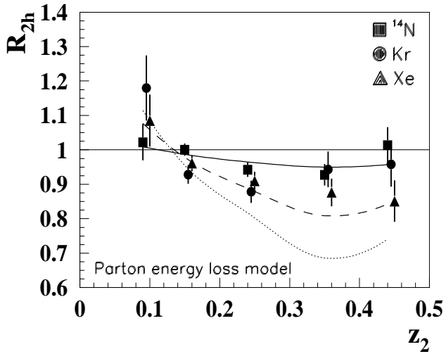
FIG. 2: The ratio R_{2h} as a function of z_2 for ^{14}\text{N} (squares), Kr (circles) and Xe (triangles) with z_1 > 0.5 for Selection II. The systematic uncertainty is 4% (3%) for xenon and krypton (nitrogen) and is independent of z_2 . The curves ( ^{14}\text{N} : solid; Kr: dashed; Xe: dotted) are from the parton energy loss model described in Refs.[16, 17].
