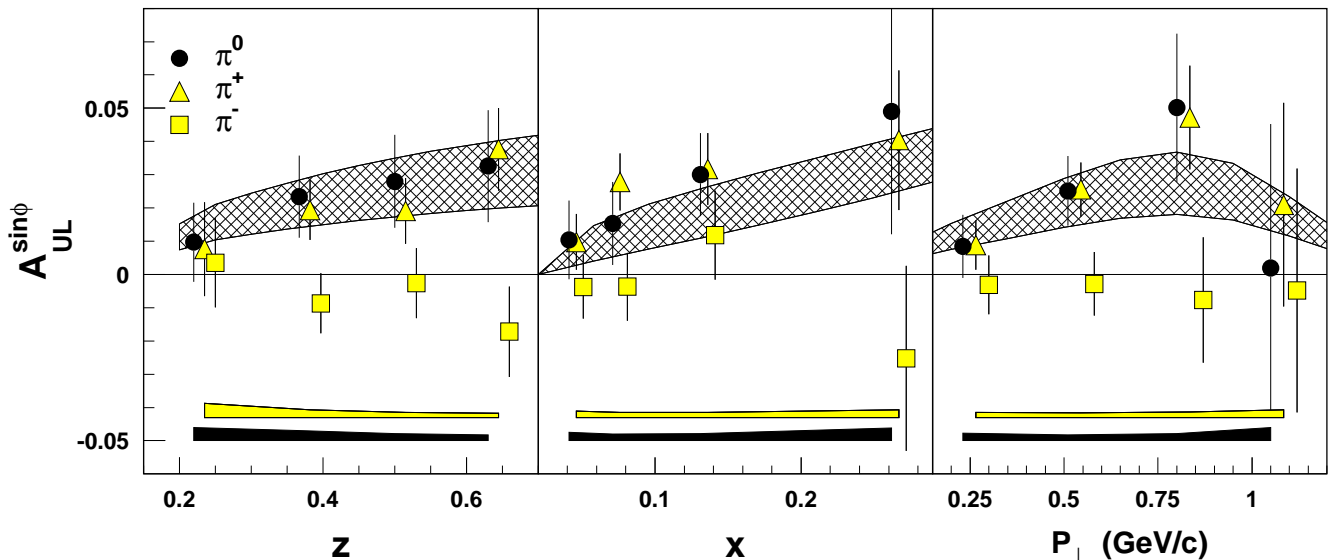
FIG. 1. Analysing power in the \sin \phi moment for \pi^0 (circles) compared to previous results [1] for \pi^+ (triangles) and \pi^- (squares) as a function of the pion fractional energy z , the Bjorken variable x , and of the pion transverse momentum P_{\perp} . Error bars include the statistical uncertainties only. The filled and open bands at the bottom of the panels represent the systematic uncertainties for neutral and charged pions, respectively. The data for charged pion production are slightly shifted in z , x , and P_{\perp} for clarity. The shaded areas show a range of predictions of a model calculation [10,17] applied to the case of \pi^0 electroproduction (see text).
